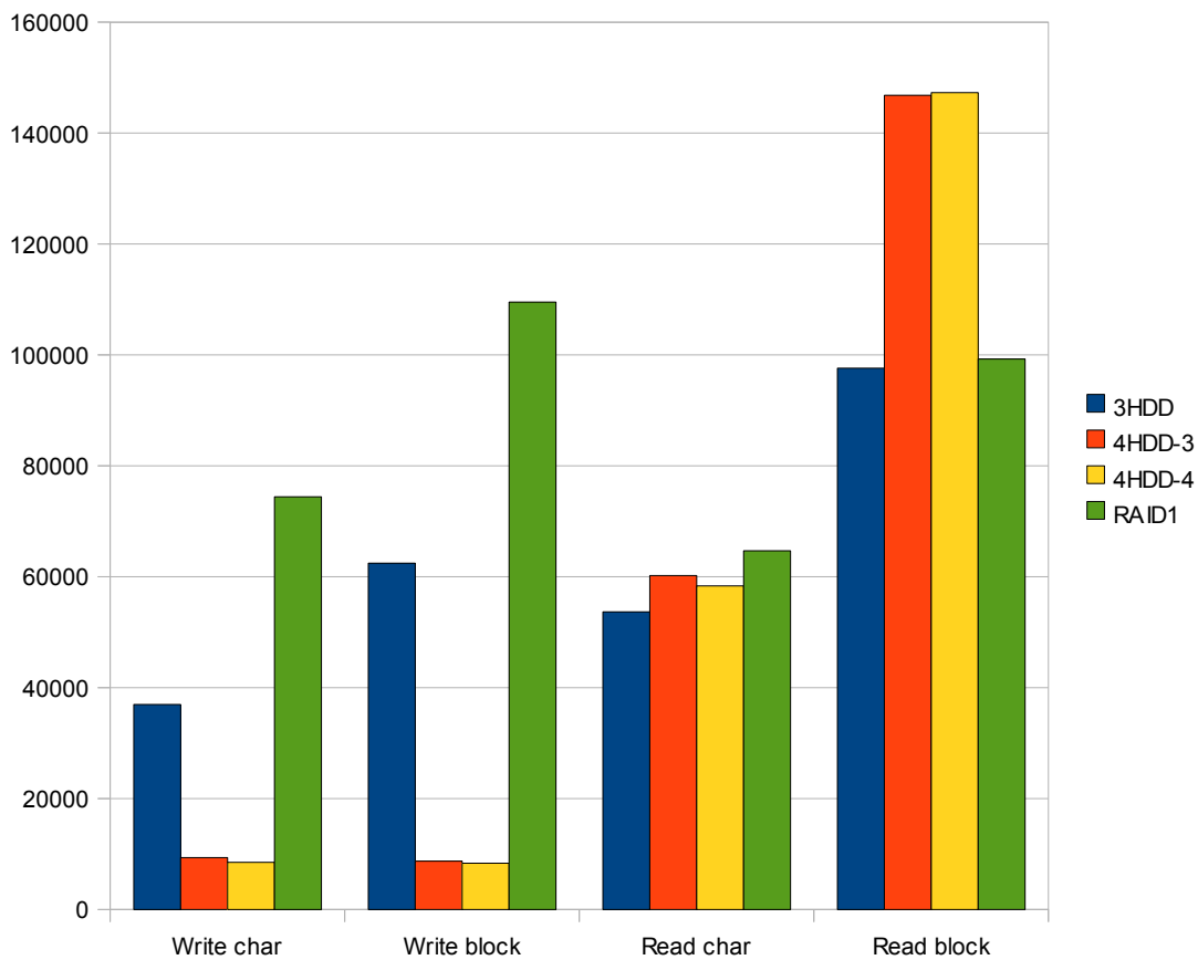
RAID comparison with stripe=32
