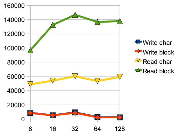
RAID5 4HDD (2048/16384 contig 3)
